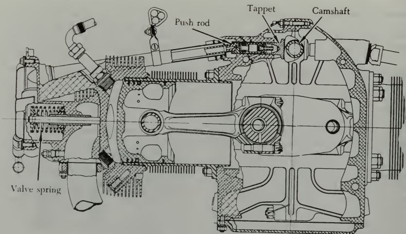
FIGURE 1-19. Valve-operating mechanism (opposed engine).
